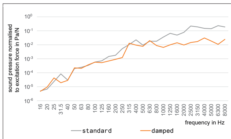
Fig 3. Excitation-normalised sound pressure of the prototype crossing when tested under laboratory conditions.
